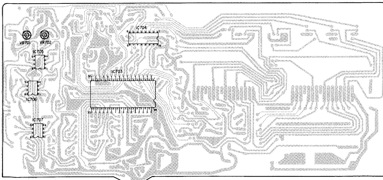
Display P. C. Board
